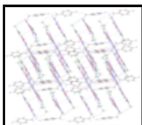
Fig. 3. Crystal packing of (I) showing the three-dimensional network, with hydrogen bonds drawn as dashed lines.
