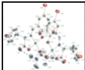
Fig. 1. The asymmetric unit of (I), with 30% probability displacement ellipsoids for non-H atoms. Hydrogen atoms have been omitted and C—H...O hydrogen bonds are drawn as dashed lines.
